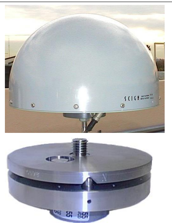
Figure 5. Custom GPS equipment for continuous GPS monitoring stations. (Top) SCIGN short antenna radome covering a GPS choking antenna; (Bottom) Adjustable antenna adapter/mount. Source: SCIGN project.
