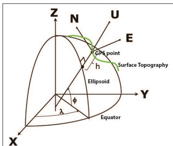
Figure 6. Coordinate systems used for deriving Epoch 2017.50. Analysis of GPS phase and pseudorange data is carried out in a global Earth-centered Earth-fixed reference frame (X,Y,Z) – here in ITRF2014. The ITRF2014 coordinates are transformed to geodetic latitude, longitude and ellipsoidal height ( \phi , \lambda , h ) with respect to a geocentric oblate ellipsoid of revolution (one octant shown) – here the WGS84 ellipsoid. Transformation of positions in the right-handed (X,Y,Z) frame to displacements in a left-handed local frame ( \Delta N, \Delta E, \Delta U ) is a function of geodetic latitude and longitude (equation 1). Source: Bock and Melgar (2016).
