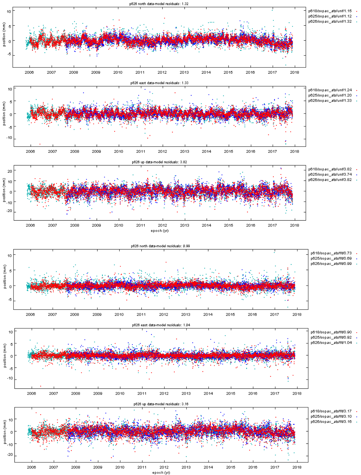
Figure 8. (Top) Overlay unfiltered displacement time series for 3 CSRN stations showing “common-mode” periodic features; (Bottom) Filtered displacement time series showing a significant decrease in scatter (wrms) in the horizontal components and less so for the vertical component Source: Source: GPS Explorer Time Series Applet ( http://geoexp01.ucsd.edu/gridsphere/gridsphere ).
