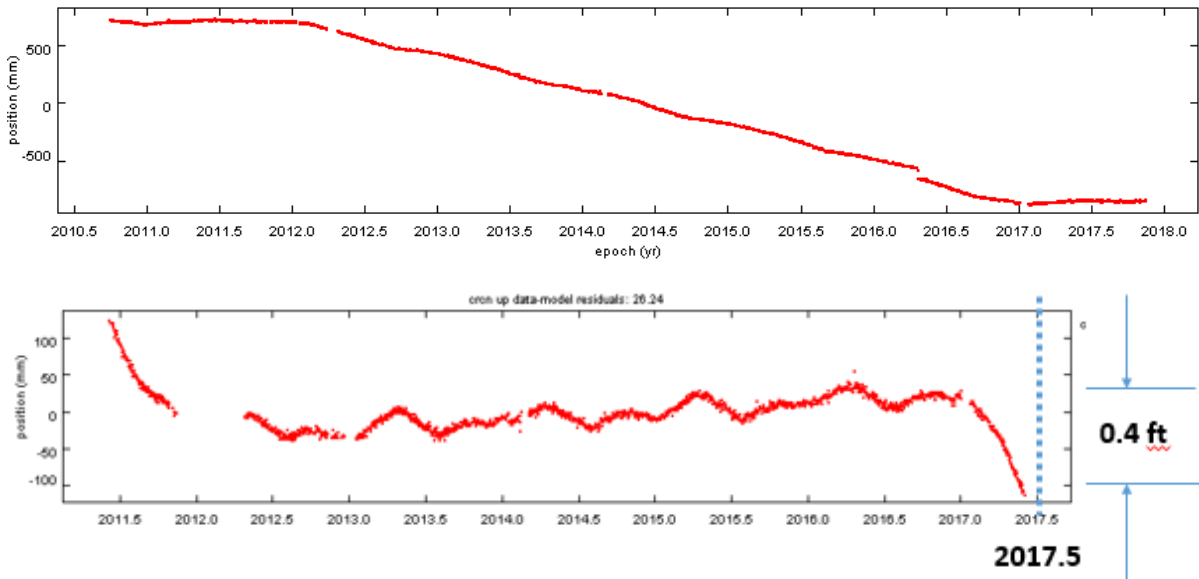
Figure 10. (Top) Raw up time series for CVSRN station CRCN in the southern part of the Central Valley. (Bottom). Residuals after fitting the up time series with a single slope. The residuals diverge at the ends because of the change in subsidence rate at about 2012.3 and at about 2017.0. Source: GPS Explorer Time Series Applet ( http://geoexp01.ucsd.edu/gridsphere/gridsphere ).
